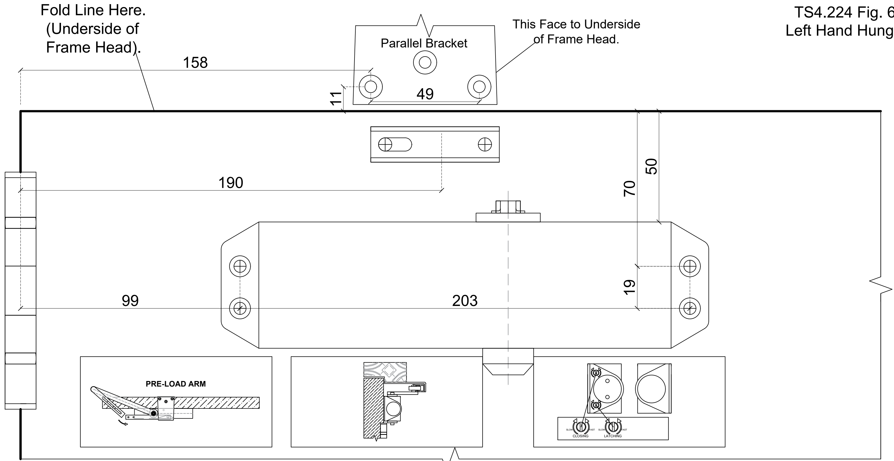
This Template Covers Regular Parallel Arm Installation to 105°
